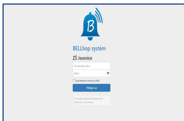
Program BELLHop
